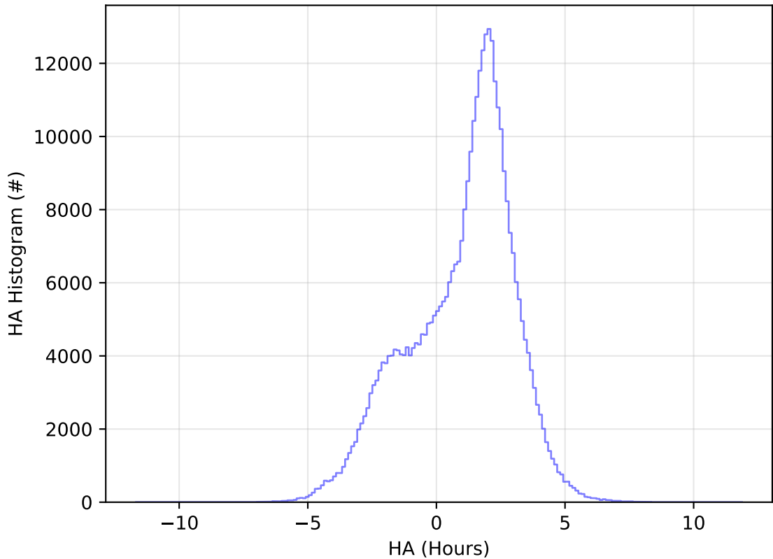
early_u_fpextra3.0_v3.4_10yrs All sky y band: HA Histogram
