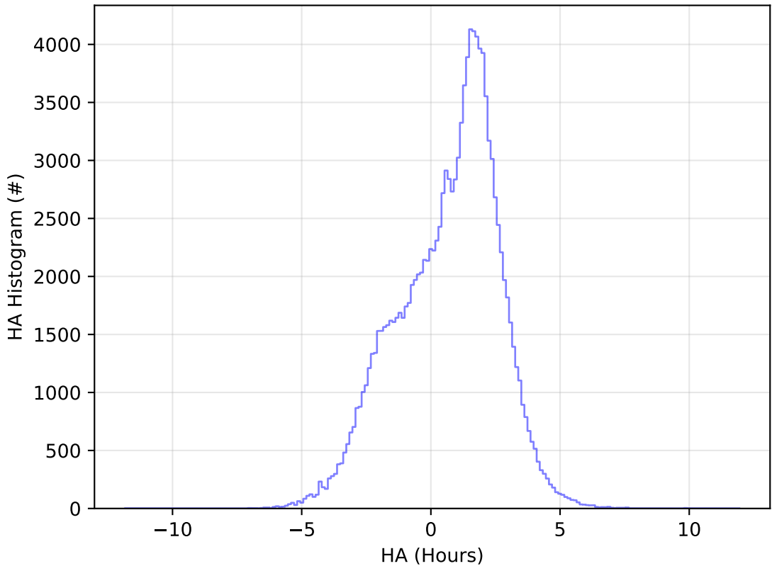
early_u_fpextra3.0_v3.4_10yrs All sky u band: HA Histogram
