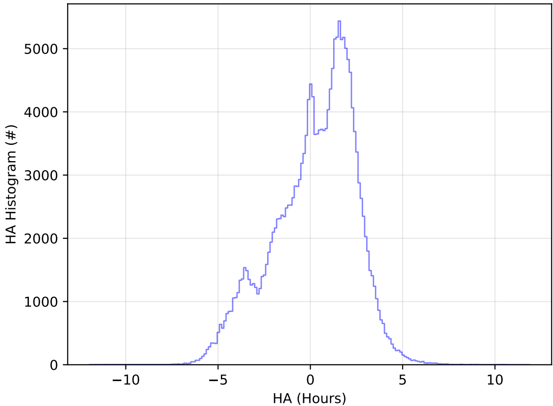
early_u_fpextra3.0_v3.4_10yrs All sky g band: HA Histogram
