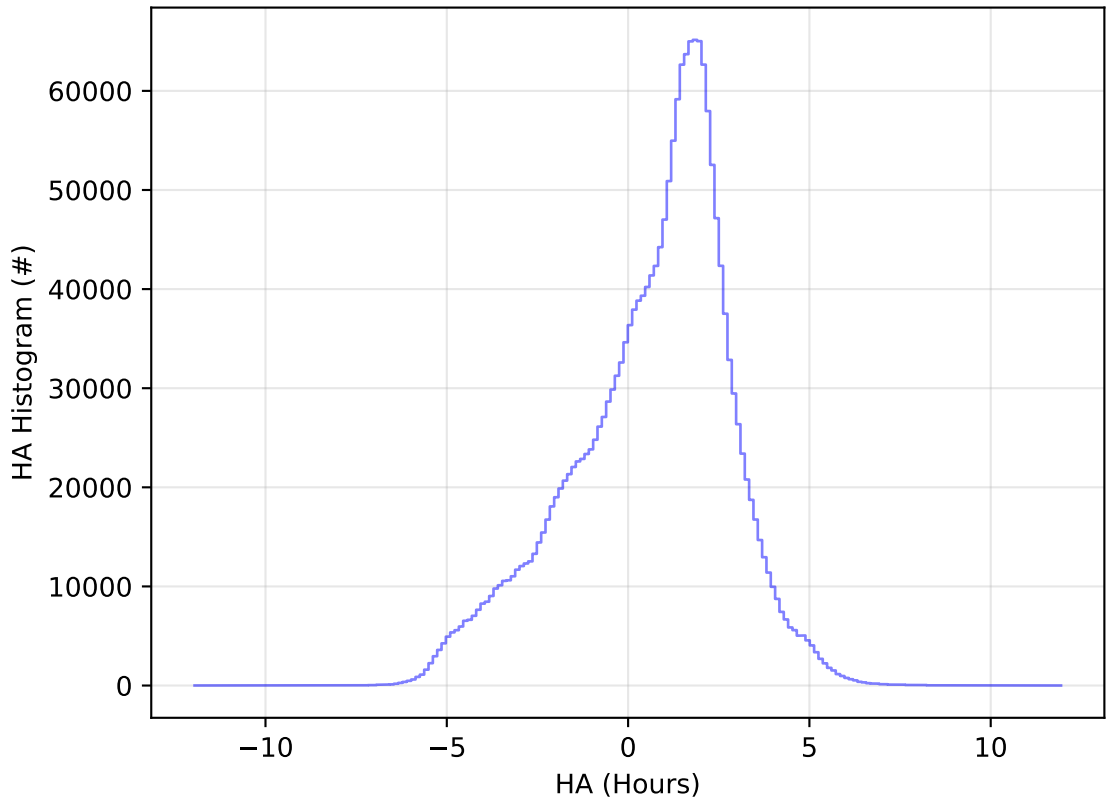
early_u_fpextra3.0_v3.4_10yrs All sky all bands: HA Histogram
