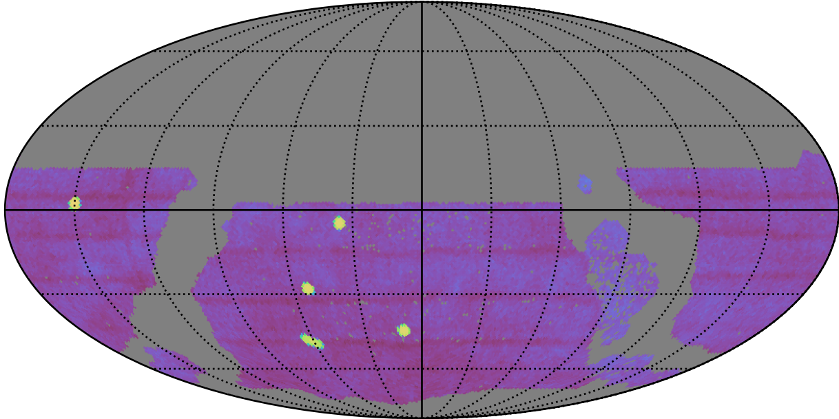
early_u_fpextra3.0_v3.4_10yrs gri WFD: Fraction of visits with a revisit < 60 min
