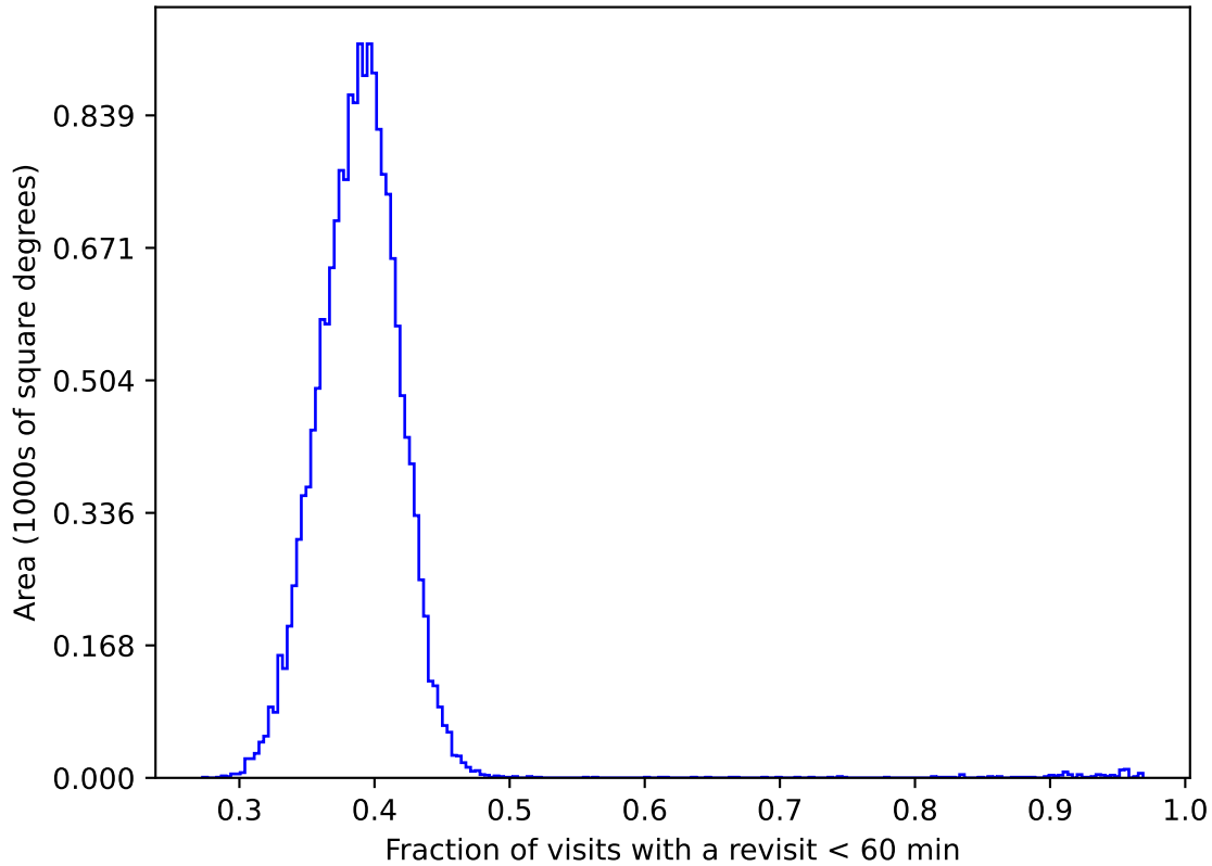
early_u_fpextra3.0_v3.4_10yrs gri WFD: Fraction of visits with a revisit < 60 min
