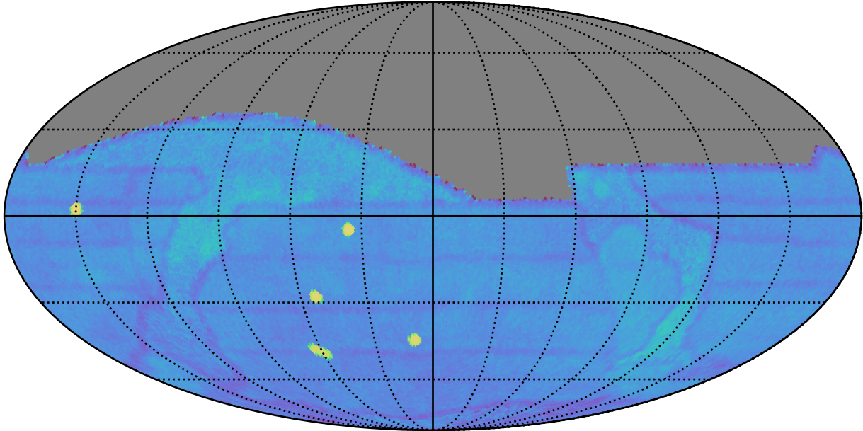
early_u_fpextra3.0_v3.4_10yrs gri All sky: Fraction of visits with a revisit < 60 min
