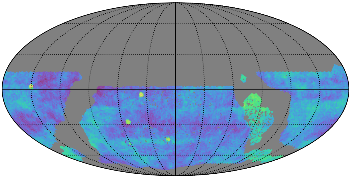
early_u_fpextra3.0_v3.4_10yrs gri WFD: Fraction of visits in pairs (20-90 min)
