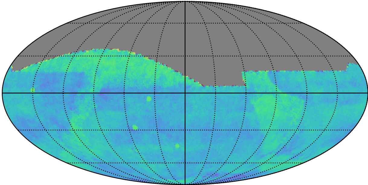
early_u_fpextra3.0_v3.4_10yrs gri All sky: Fraction of visits in pairs (20-90 min)
