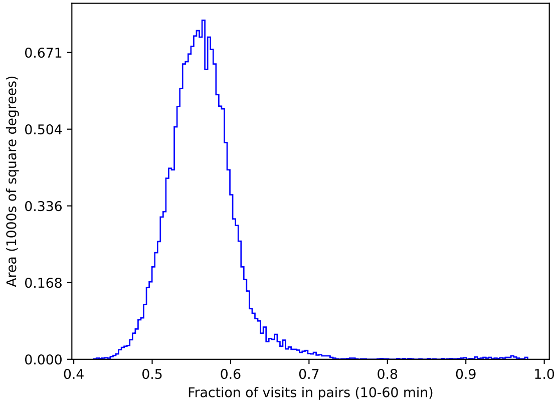
early_u_fpextra3.0_v3.4_10yrs gri WFD: Fraction of visits in pairs (10-60 min)
