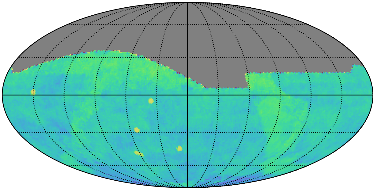
early_u_fpextra3.0_v3.4_10yrs gri All sky: Fraction of visits in pairs (10-60 min)
