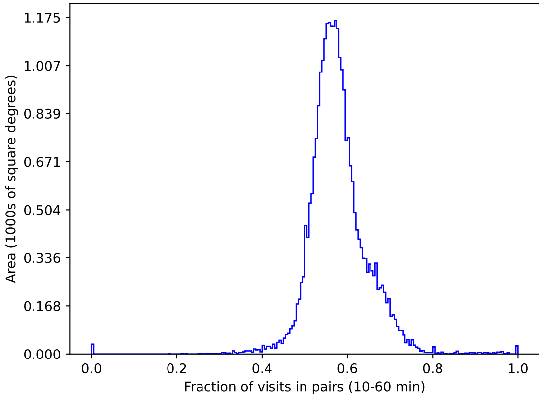
early_u_fpextra3.0_v3.4_10yrs gri All sky: Fraction of visits in pairs (10-60 min)
