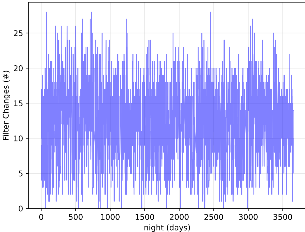
early_u_fpextra3.0_v3.4_10yrs Per Night: Filter Changes
