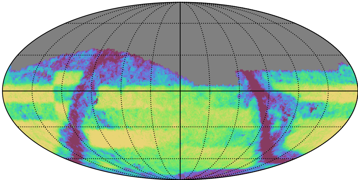
early_u_fpextra3.0_v3.4_10yrs Yr 3-4 z band: Exgal_CoaddM5
