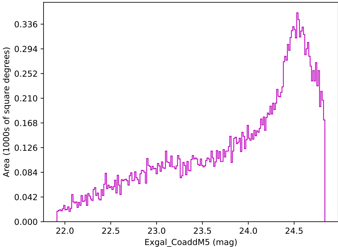
early_u_fpextra3.0_v3.4_10yrs Yr 3-4 z band: Exgal_CoaddM5
