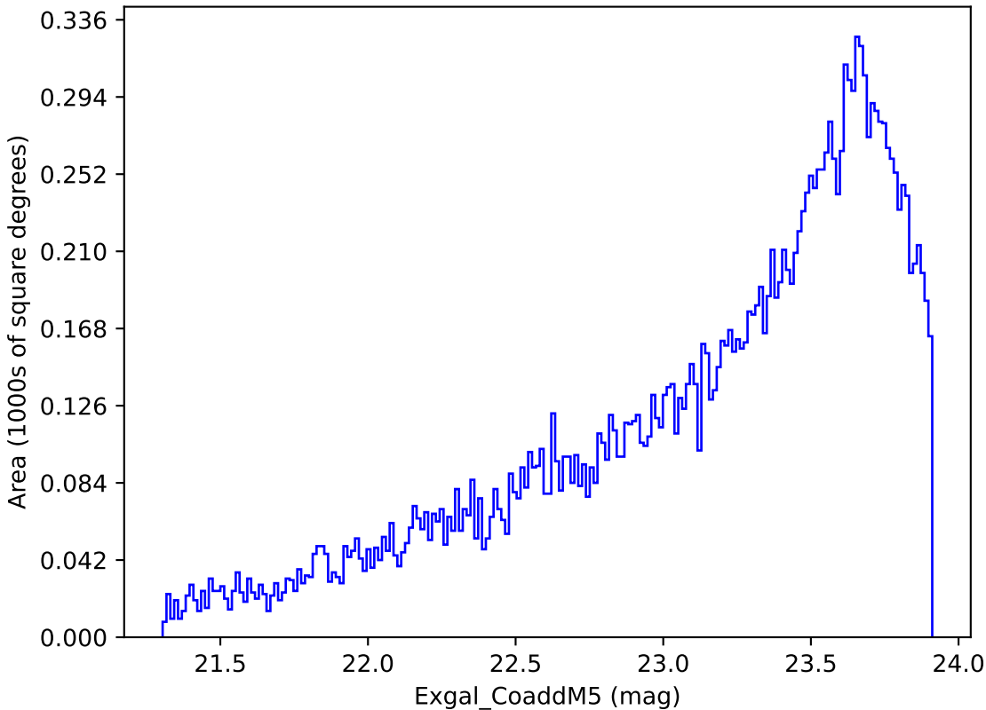
early_u_fpextra3.0_v3.4_10yrs Yr 3-4 y band: Exgal_CoaddM5
