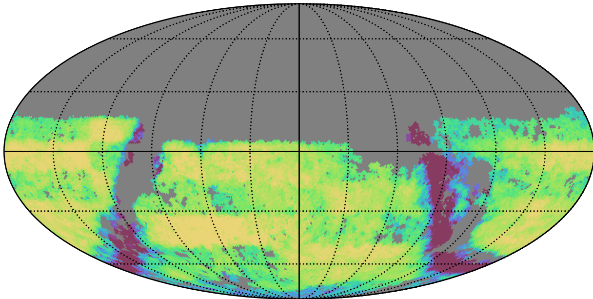
early_u_fpextra3.0_v3.4_10yrs Yr 3-4 u band: Exgal_CoaddM5
