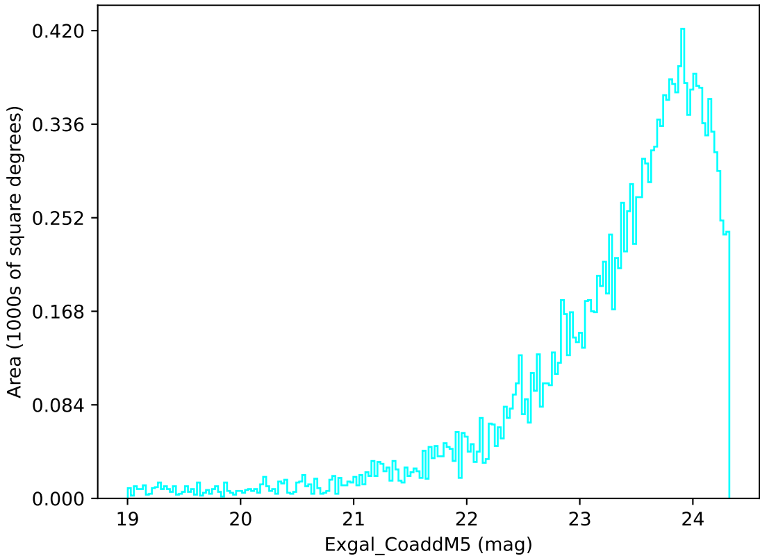
early_u_fpextra3.0_v3.4_10yrs Yr 3-4 u band: Exgal_CoaddM5
