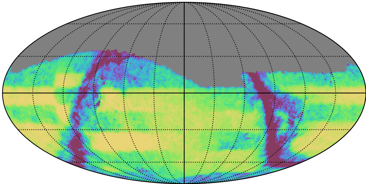
early_u_fpextra3.0_v3.4_10yrs Yr 3-4 r band: Exgal_CoaddM5
