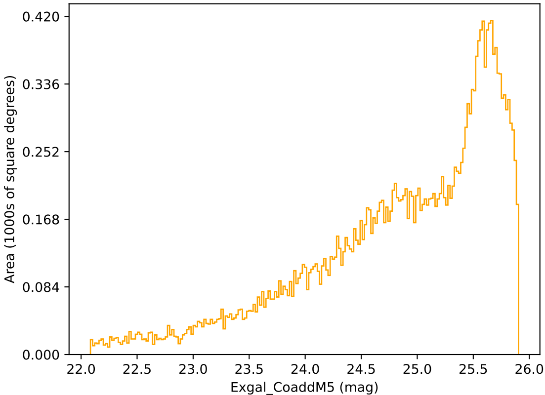
early_u_fpextra3.0_v3.4_10yrs Yr 3-4 r band: Exgal_CoaddM5
