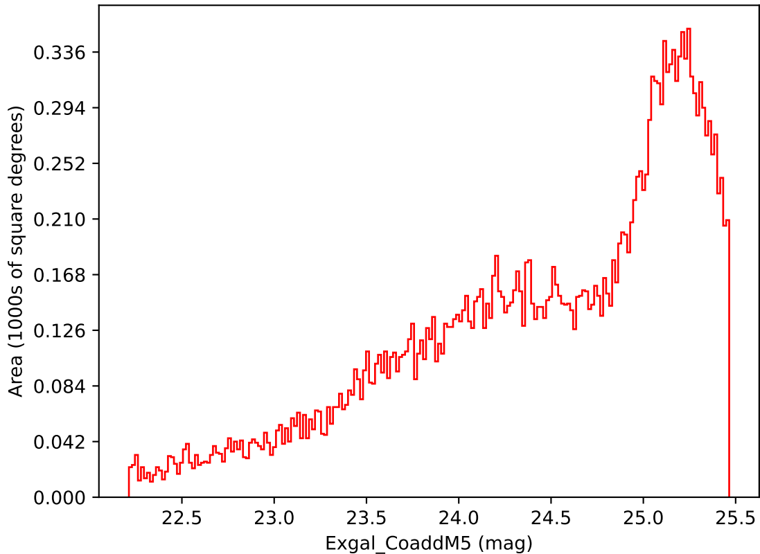
early_u_fpextra3.0_v3.4_10yrs Yr 3-4 i band: Exgal_CoaddM5
