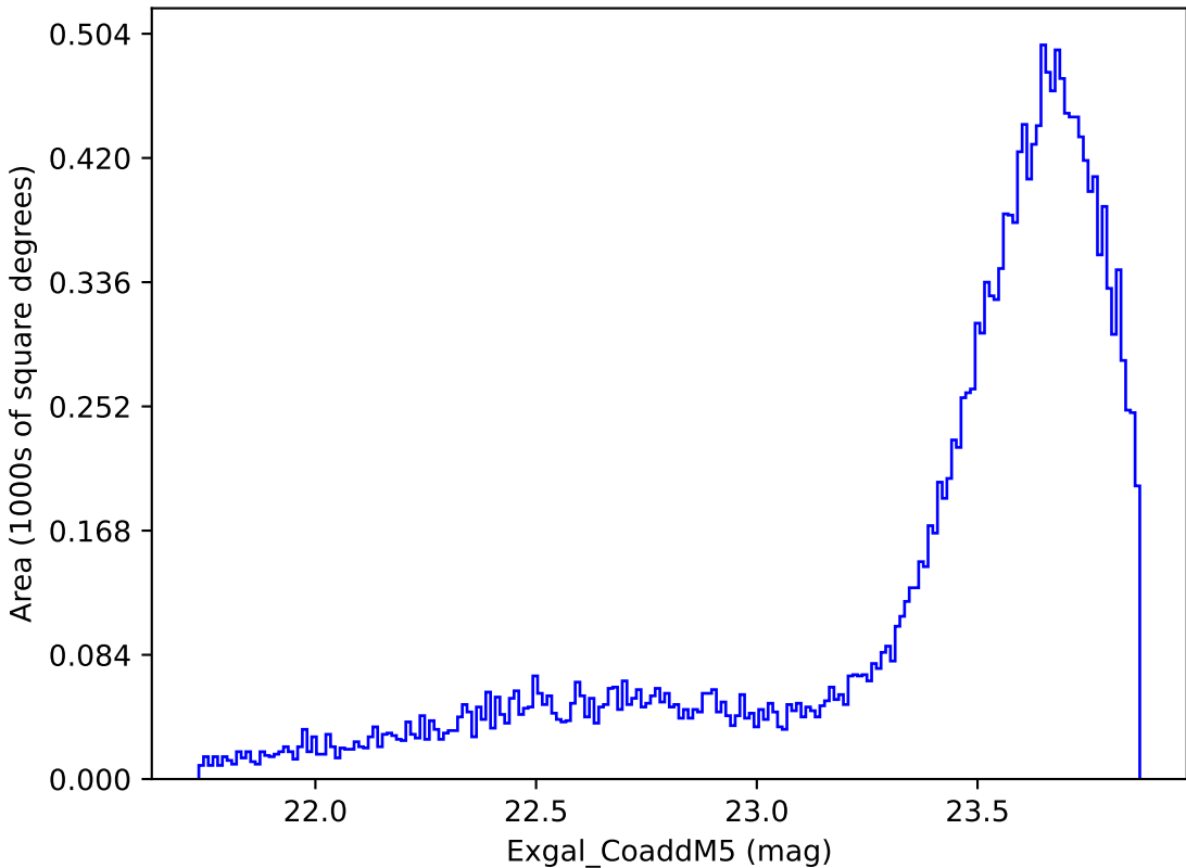
early_u_fpextra3.0_v3.4_10yrs Yr 1 y band: Exgal_CoaddM5
