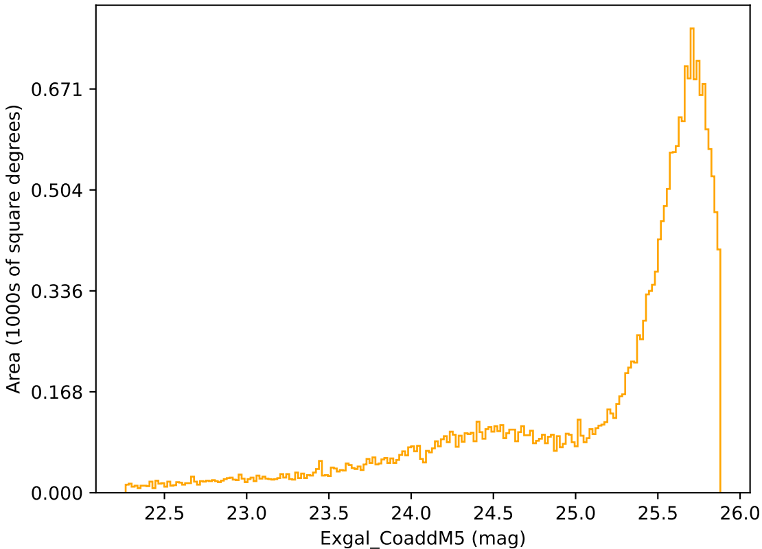
early_u_fpextra3.0_v3.4_10yrs Yr 1 r band: Exgal_CoaddM5
