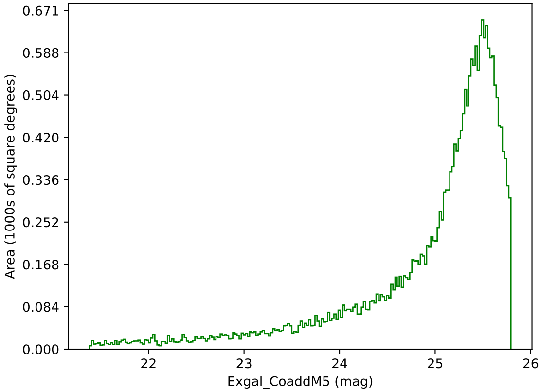
early_u_fpextra3.0_v3.4_10yrs Yr 1 g band: Exgal_CoaddM5
