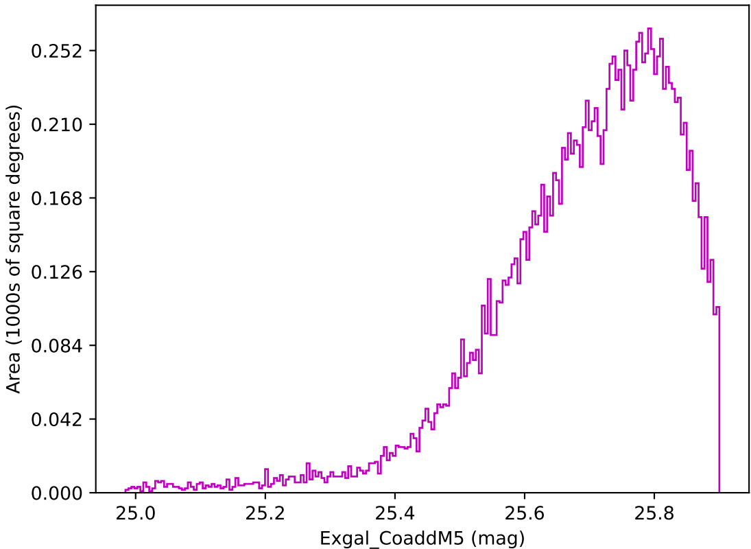
early_u_fpextra3.0_v3.4_10yrs WFD z band: Exgal_CoaddM5
