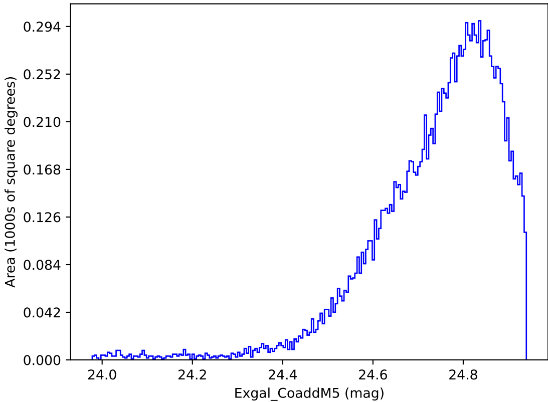
early_u_fpextra3.0_v3.4_10yrs WFD y band: Exgal_CoaddM5
