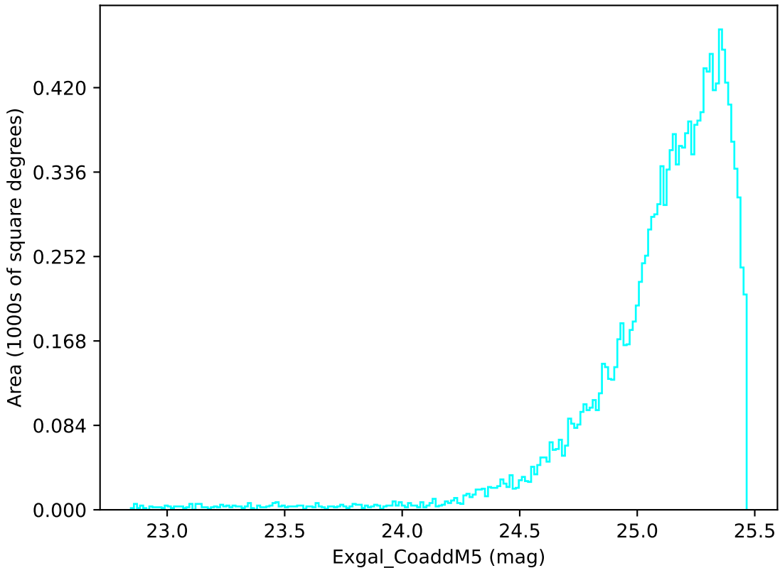
early_u_fpextra3.0_v3.4_10yrs WFD u band: Exgal_CoaddM5
