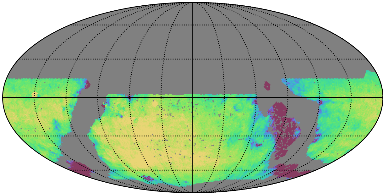
early_u_fpextra3.0_v3.4_10yrs WFD g band: Exgal_CoaddM5
