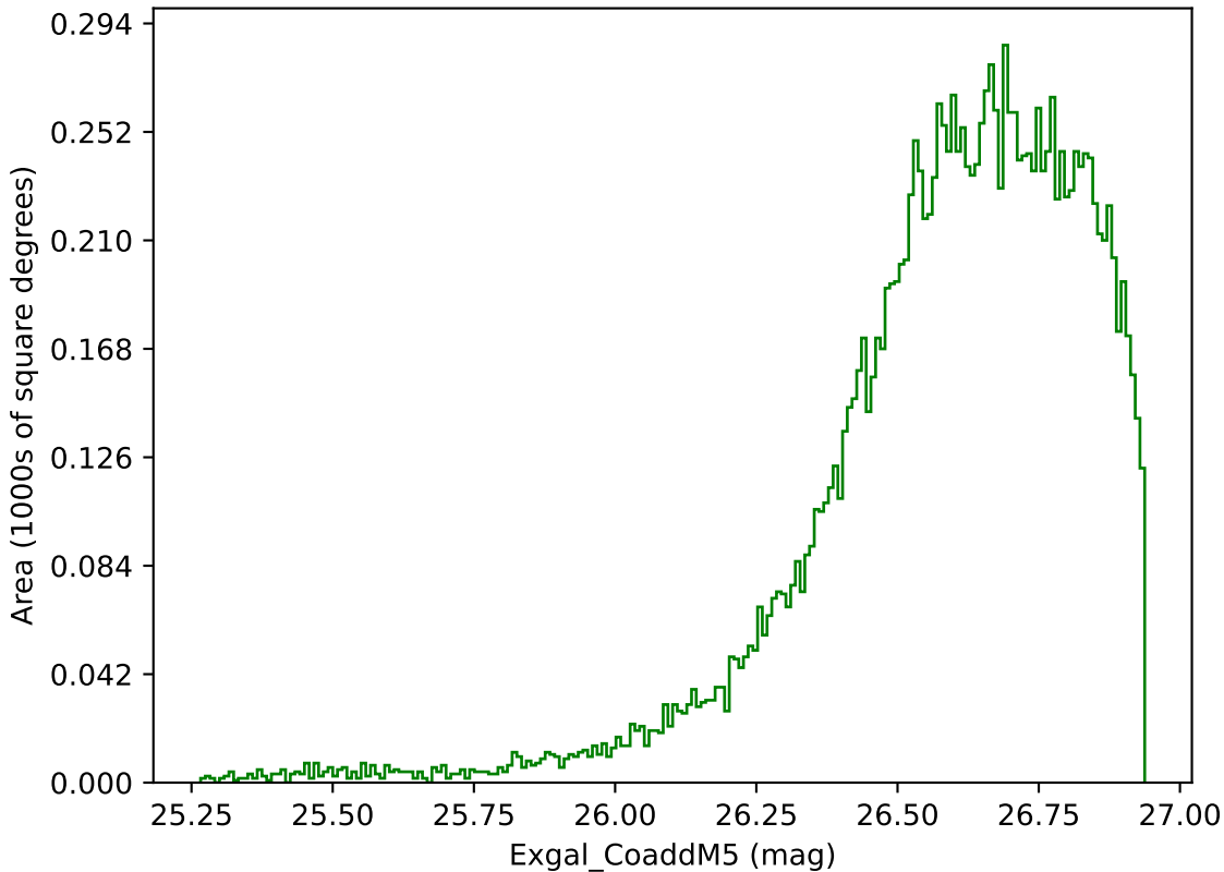
early_u_fpextra3.0_v3.4_10yrs WFD g band: Exgal_CoaddM5
