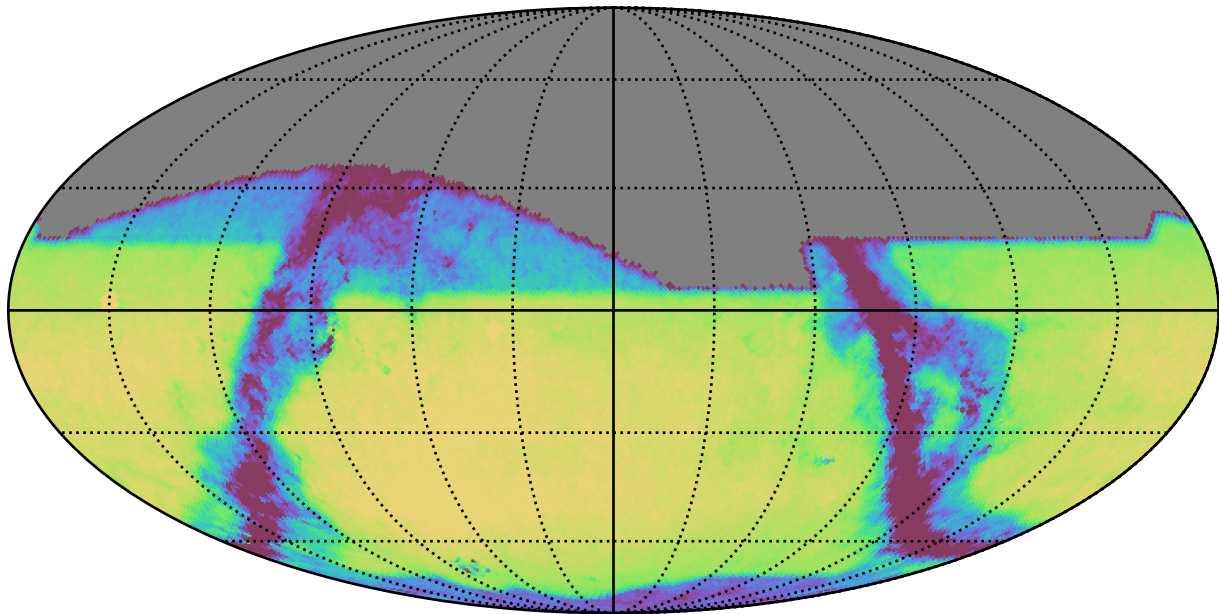
early_u_fpextra3.0_v3.4_10yrs All sky z band: Exgal_CoaddM5
