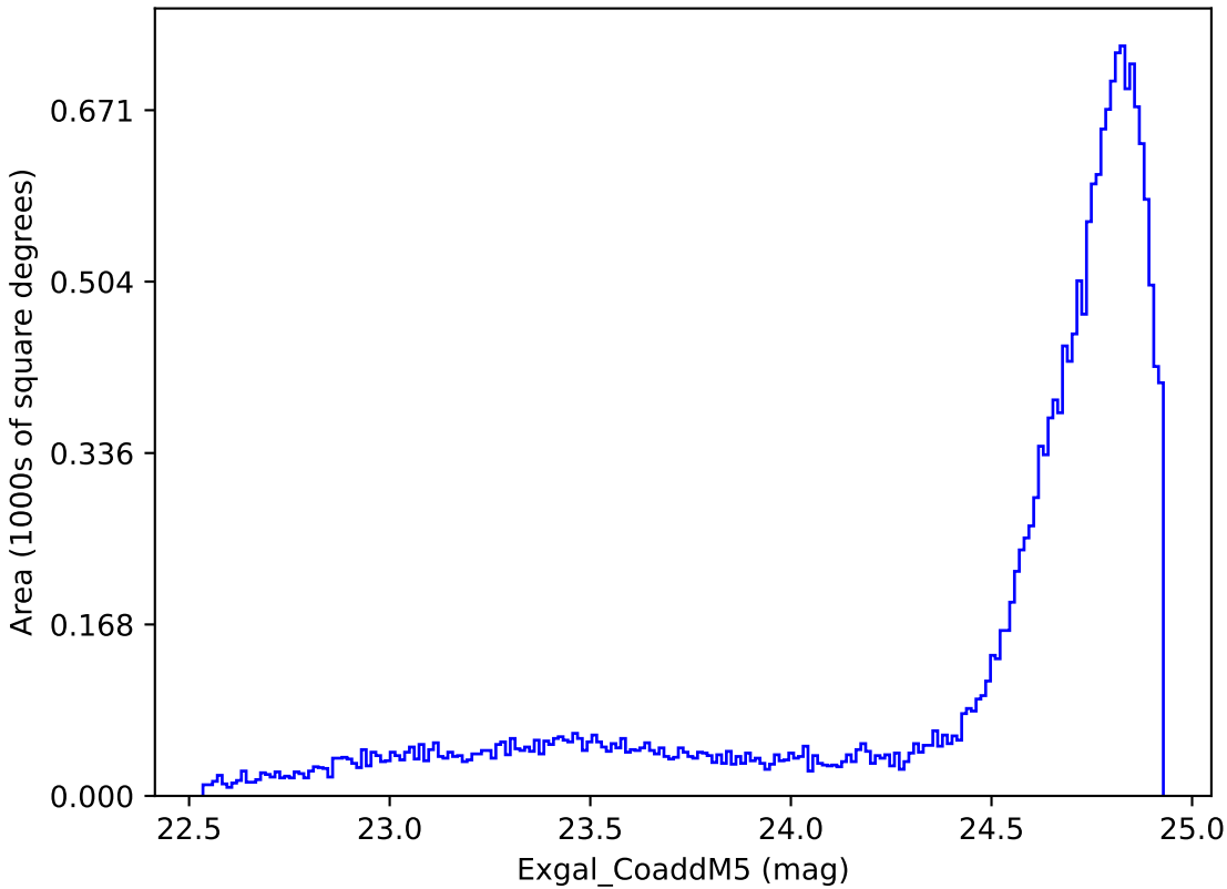
early_u_fpextra3.0_v3.4_10yrs All sky y band: Exgal_CoaddM5
