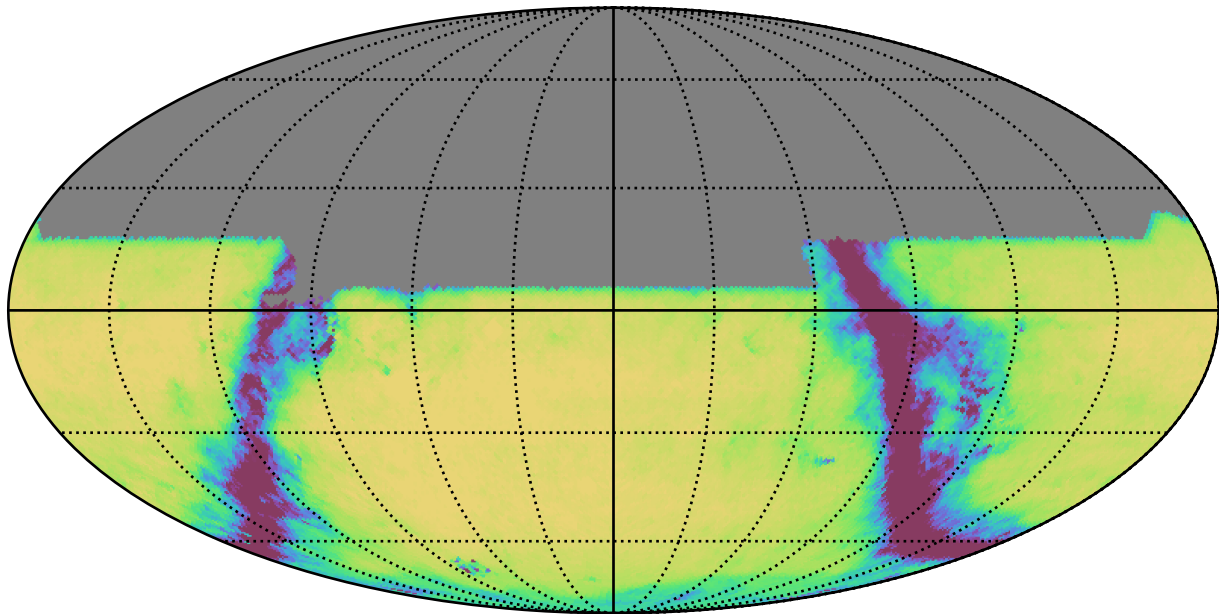
early_u_fpextra3.0_v3.4_10yrs All sky u band: Exgal_CoaddM5
