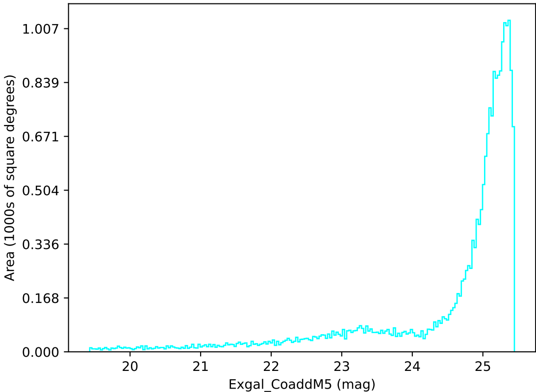
early_u_fpextra3.0_v3.4_10yrs All sky u band: Exgal_CoaddM5
