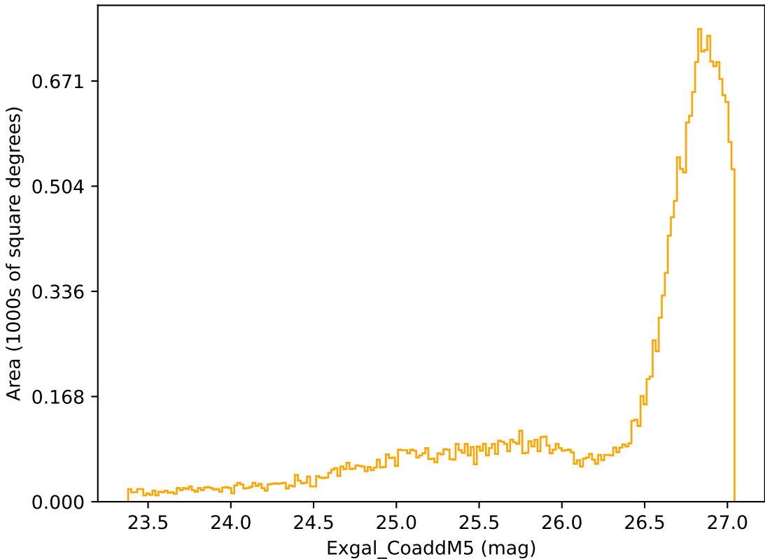
early_u_fpextra3.0_v3.4_10yrs All sky r band: Exgal_CoaddM5
