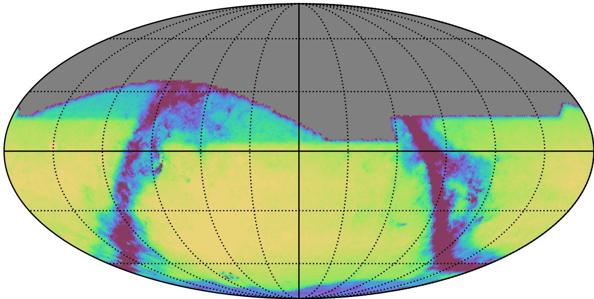
early_u_fpextra3.0_v3.4_10yrs All sky i band: Exgal_CoaddM5
