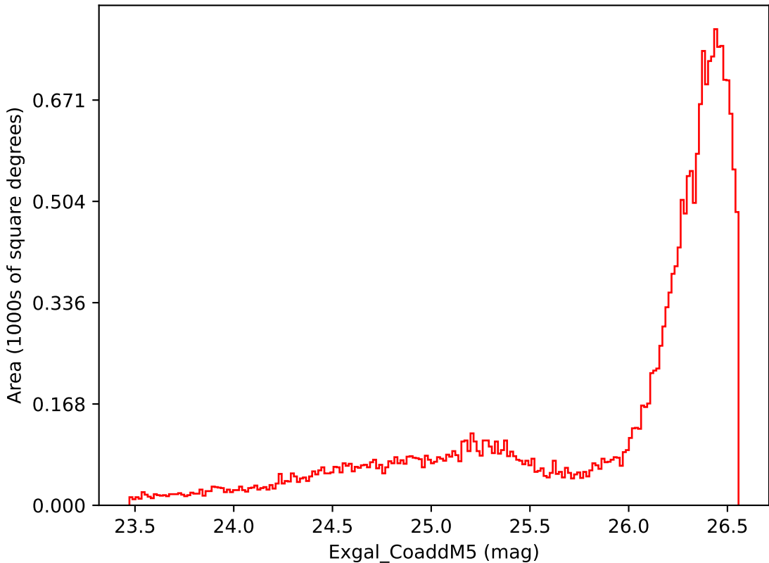
early_u_fpextra3.0_v3.4_10yrs All sky i band: Exgal_CoaddM5
