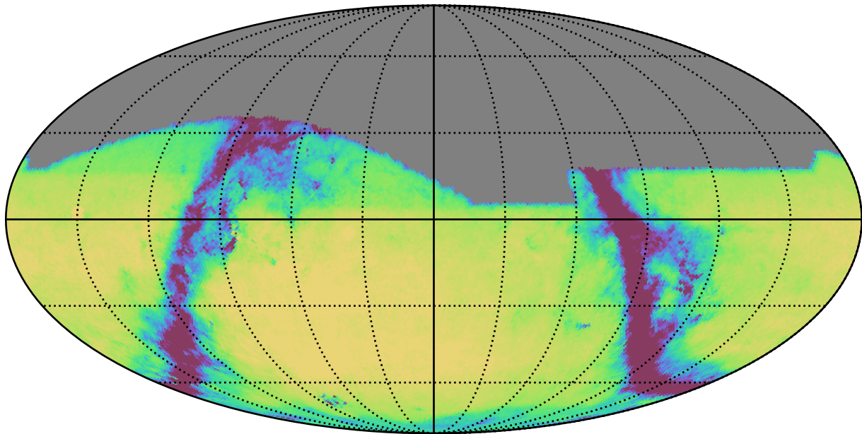
early_u_fpextra3.0_v3.4_10yrs All sky g band: Exgal_CoaddM5
