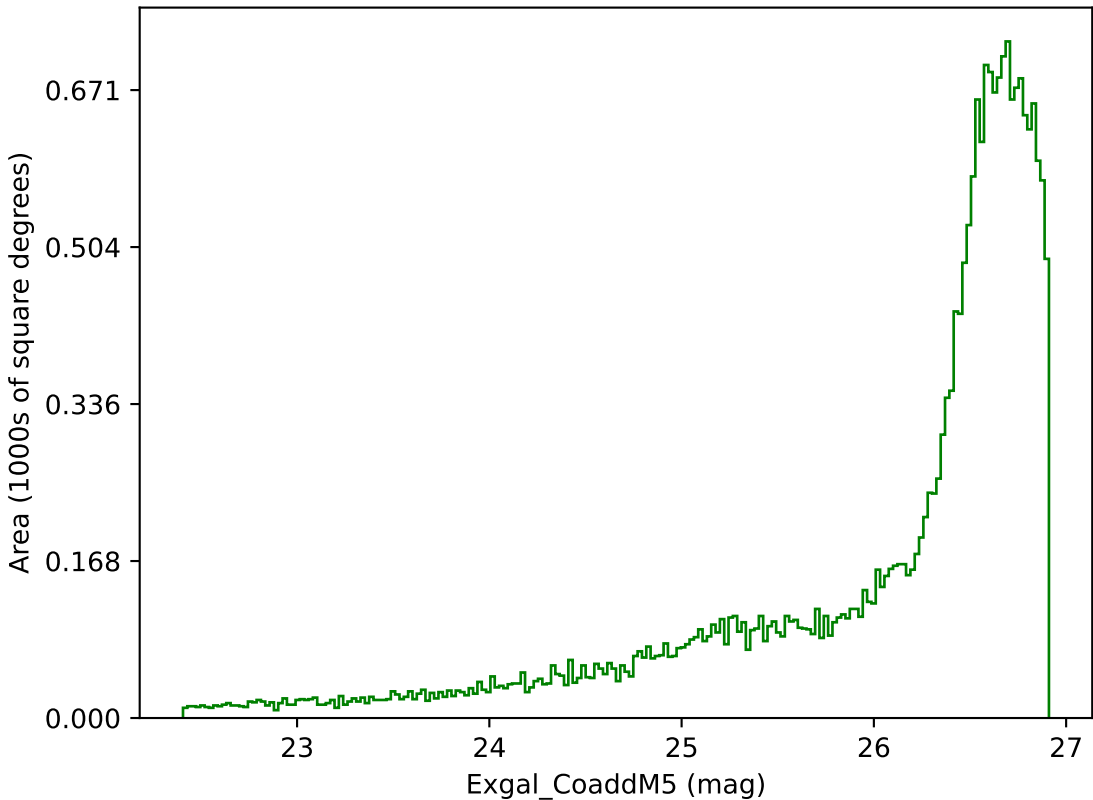
early_u_fpextra3.0_v3.4_10yrs All sky g band: Exgal_CoaddM5
