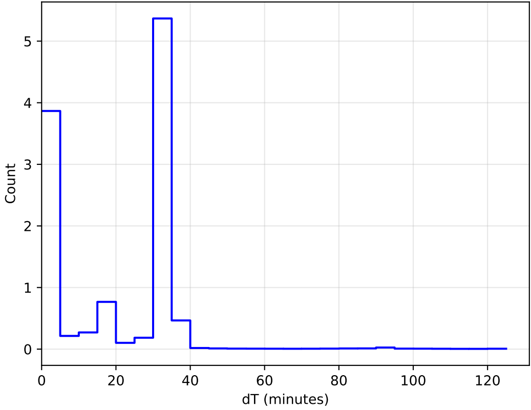
early_u_fpextra3.0_v3.4_10yrs WFD: DeltaT Histogram
