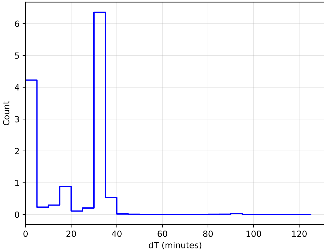
early_u_fpextra3.0_v3.4_10yrs All sky: DeltaT Histogram
