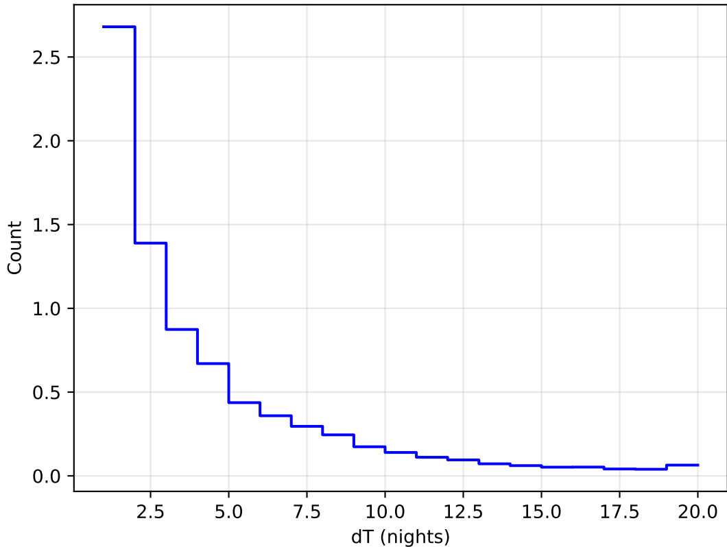
early_u_fpextra3.0_v3.4_10yrs WFD all bands: DeltaNight Histogram 1e6
