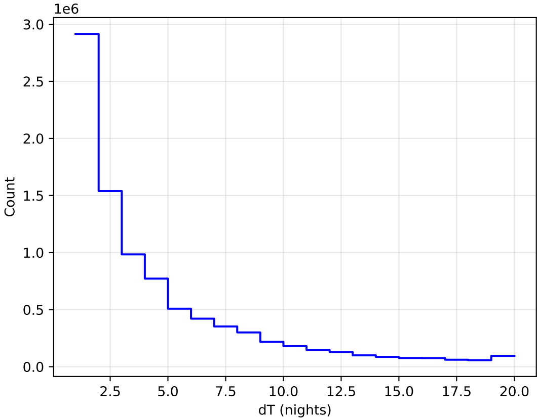
early_u_fpextra3.0_v3.4_10yrs All sky all bands: DeltaNight Histogram
