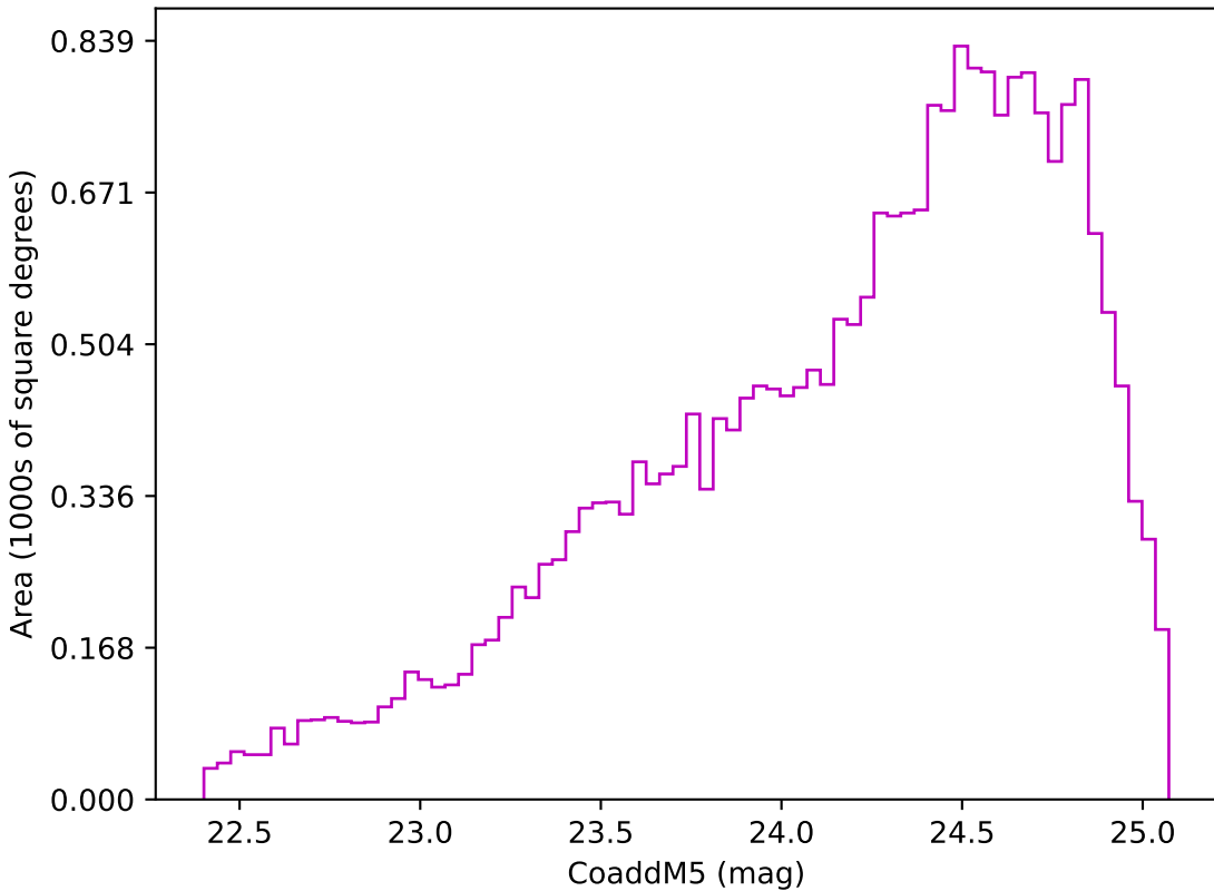
early_u_fpxextra3.0_v3.4_10yrs Yr 3-4 z band: CoaddM5
