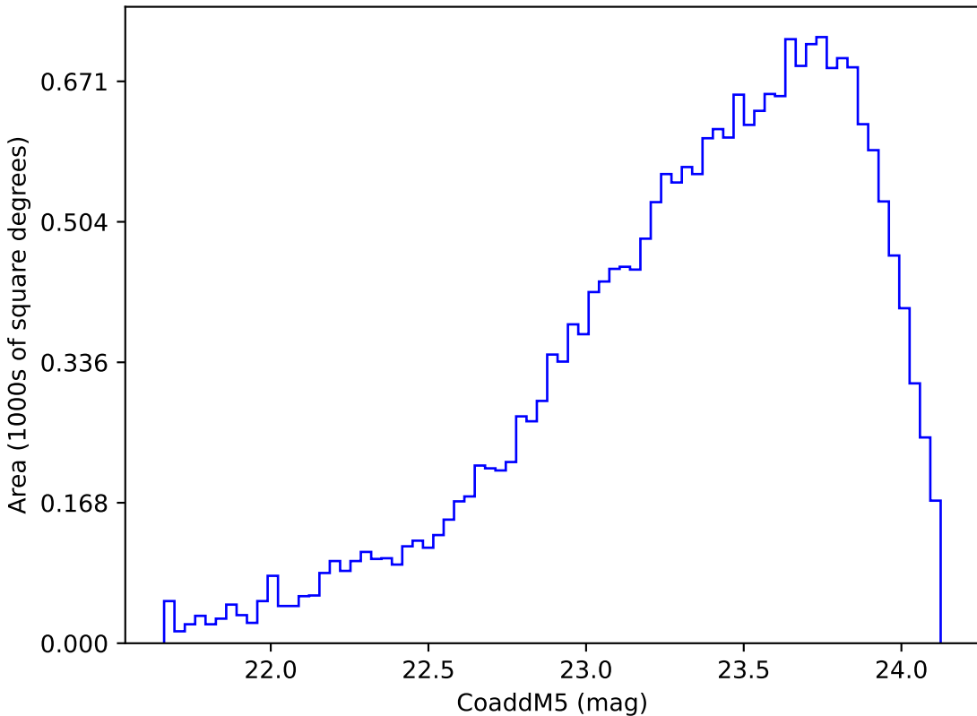
early_u_fpextra3.0_v3.4_10yrs Yr 3-4 y band: CoaddM5
