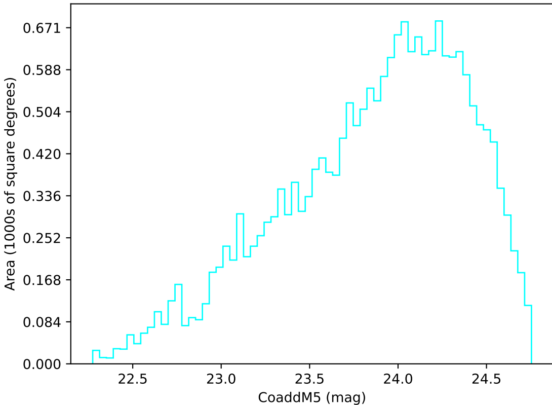
early_u_fpextra3.0_v3.4_10yrs Yr 3-4 u band: CoaddM5
