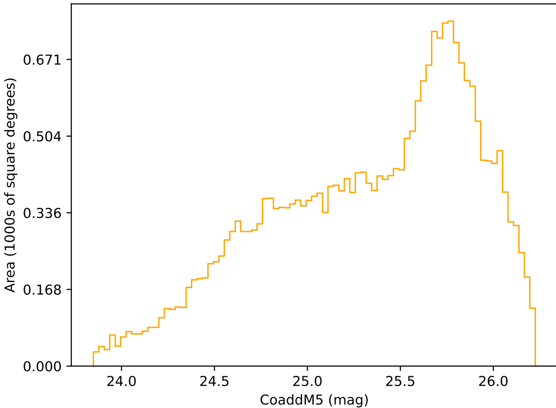
early_u_fpextra3.0_v3.4_10yrs Yr 3-4 r band: CoaddM5
