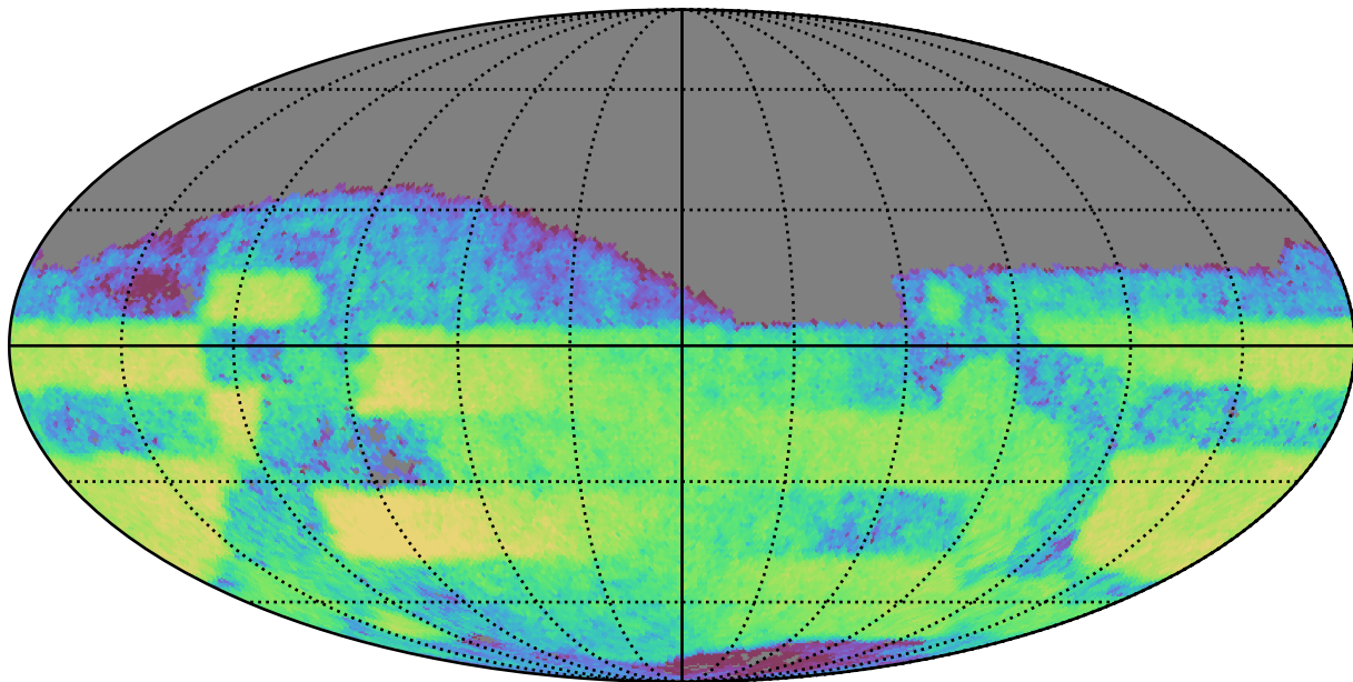
early_u_fpextra3.0_v3.4_10yrs Yr 3-4 i band: CoaddM5
