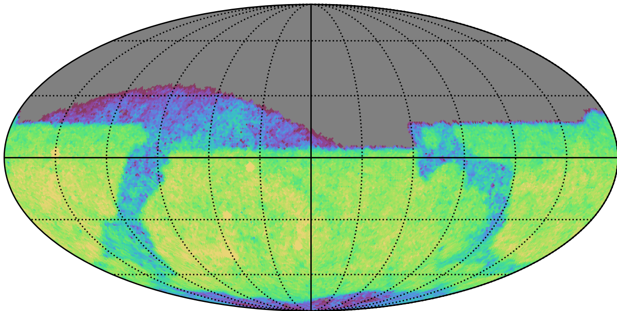
early_u_fpextra3.0_v3.4_10yrs Yr 1 z band: CoaddM5
