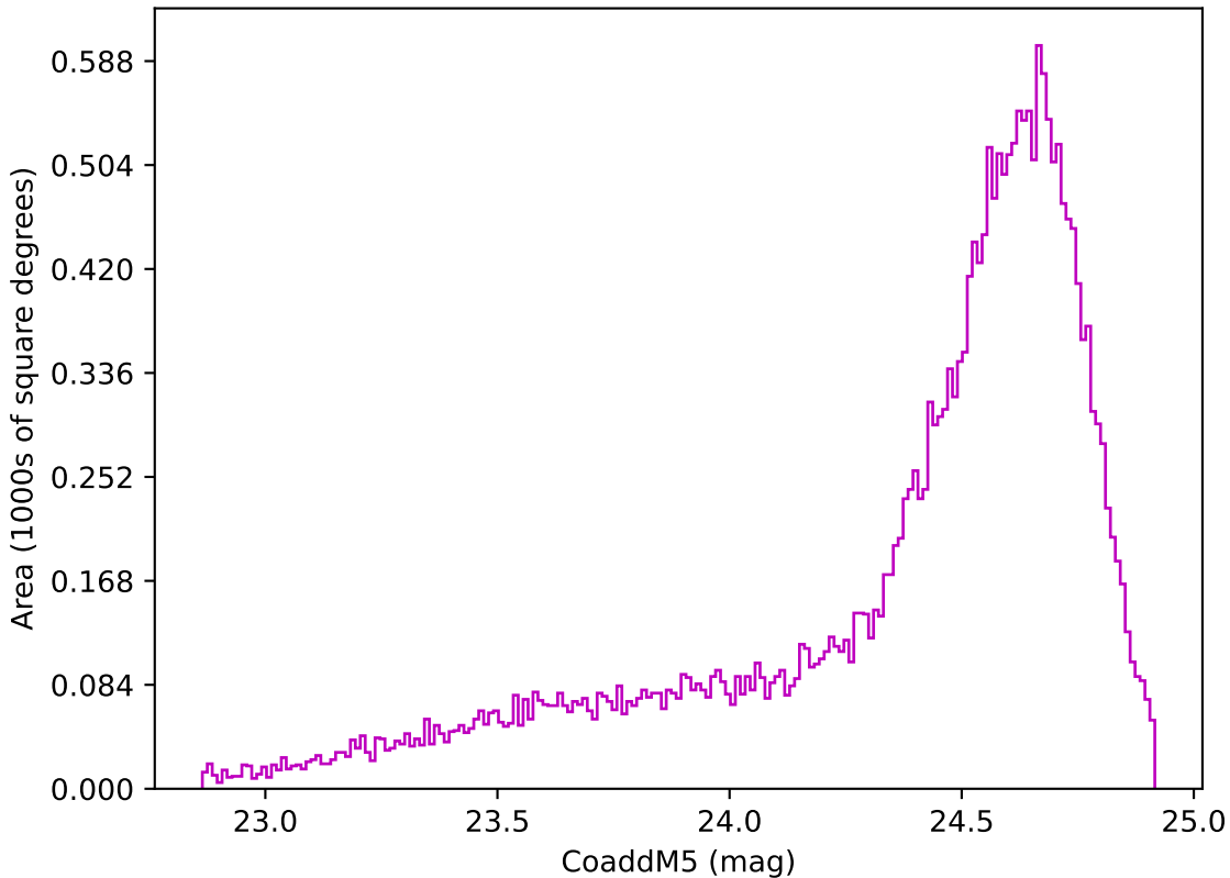
early_u_fpextra3.0_v3.4_10yrs Yr 1 z band: CoaddM5
