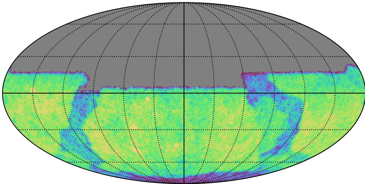
early_u_fpextra3.0_v3.4_10yrs Yr 1 y band: CoaddM5
